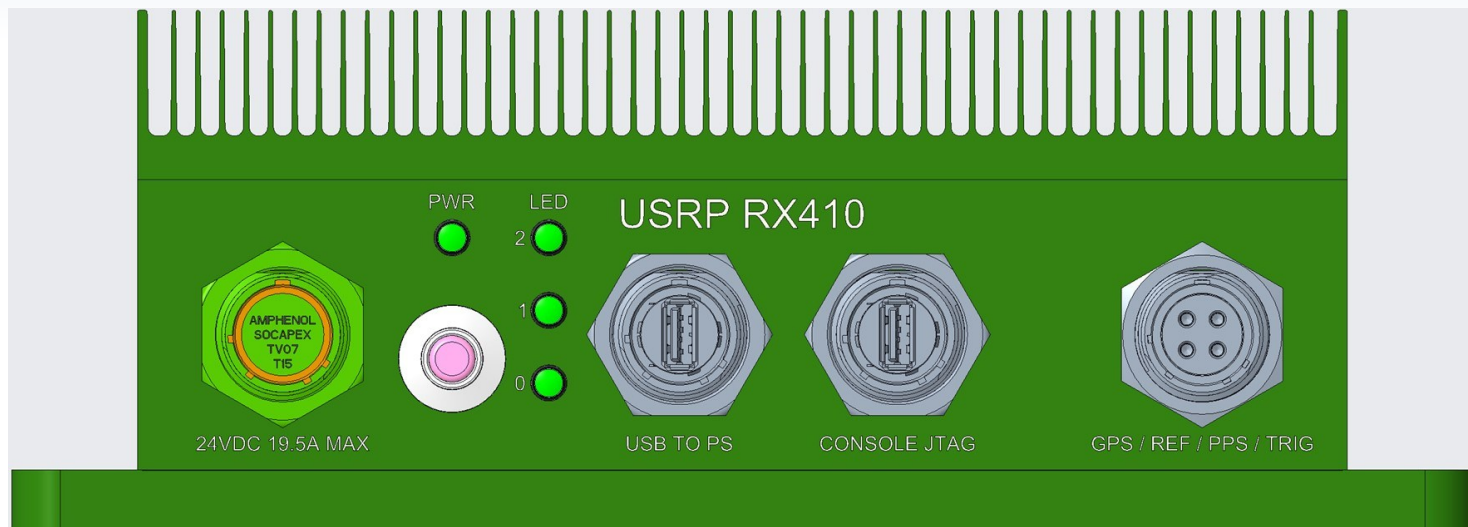
Front I/O—MIL
